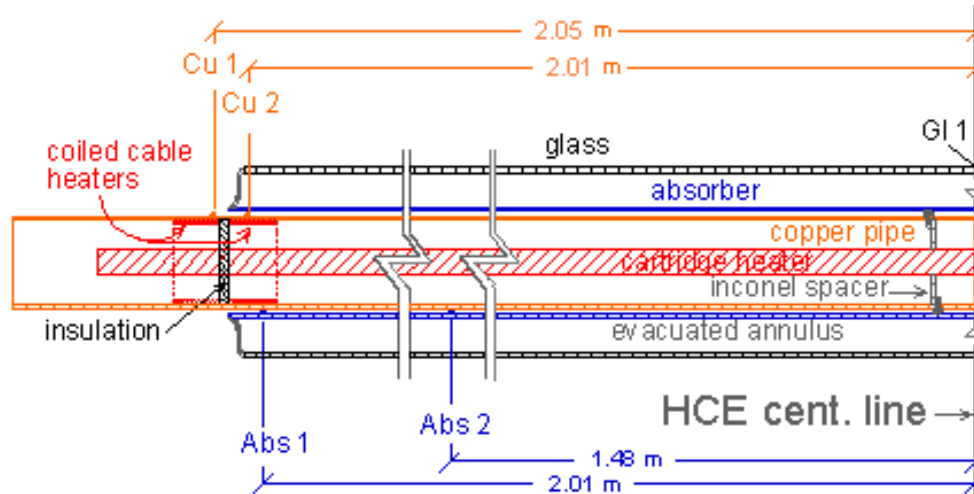
Figure 4. Copper (Cu), absorber (Abs), and glass (Gl) thermocouple locations; absorber at 25°C
