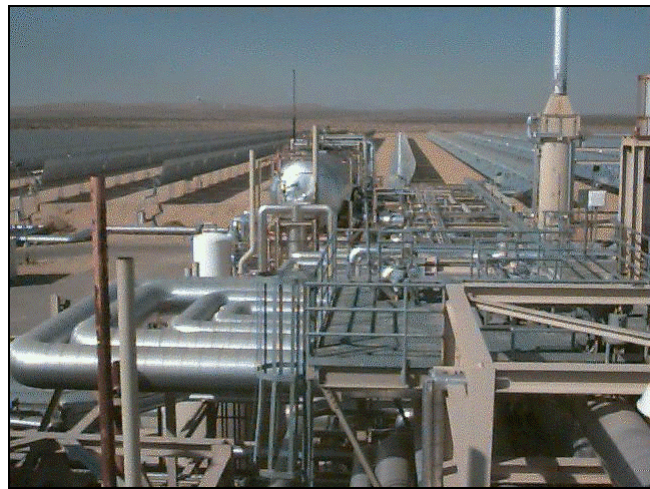
Figure 11. SEGS VI power block
