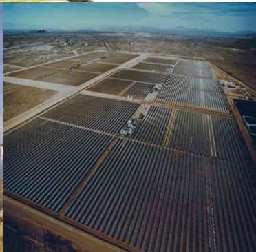
Figure 1: Above, power tower pilot project, pioneered in the U.S. (Barstow, CA) and (left) commercial unit under development by Abengoa called PS10, an 11 MW plant in Sevilla Spain (photo credit: Abengoa Solar). Bottom left, Stirling Dish/Engine, Center SEGS trough plants, Right, Compact Linear Fresnel Reflector.
