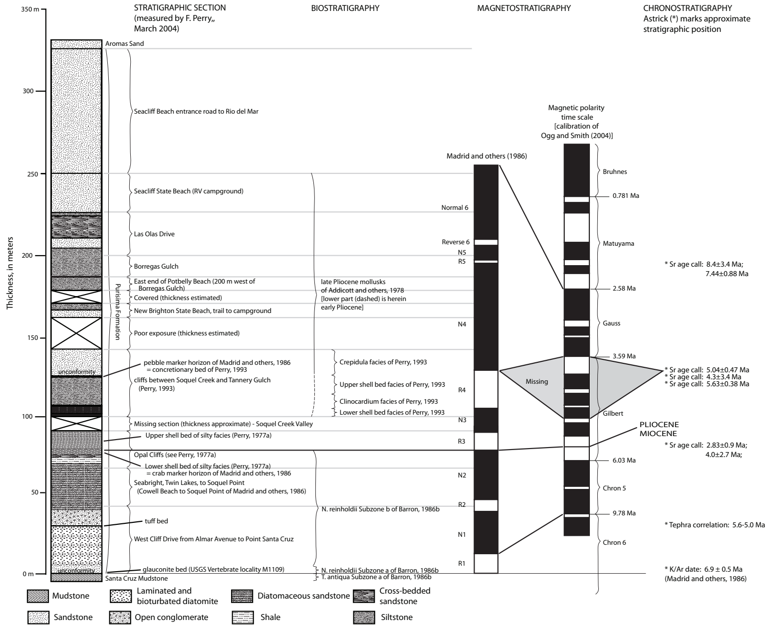
Figure 2. Supplementary reference section of the Purisima Formation along the coast between Point Santa Cruz and Rio del Mar, northern and eastern Monterey Bay, central California, showing lithostratigraphy, biostratigraphy, magnetostratigraphy, and chronostratigraphy (including tephrochronology and strontium isotope age determinations).
