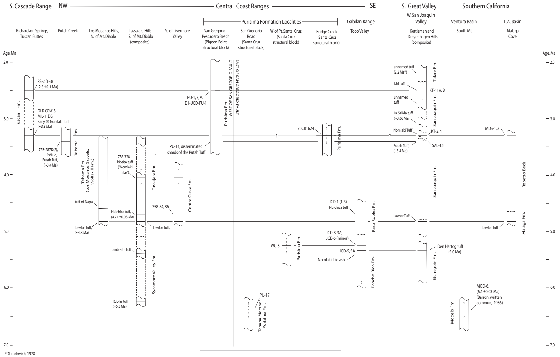
Figure 5. Chronostratigraphy of tephra found in the Purisima Formation, central California, based on tephra correlations in the Western United States. Field numbers and correlations are based on published database compiled by A.M. Sarna-Wojcicki, U.S. Geological Survey, 2005.
