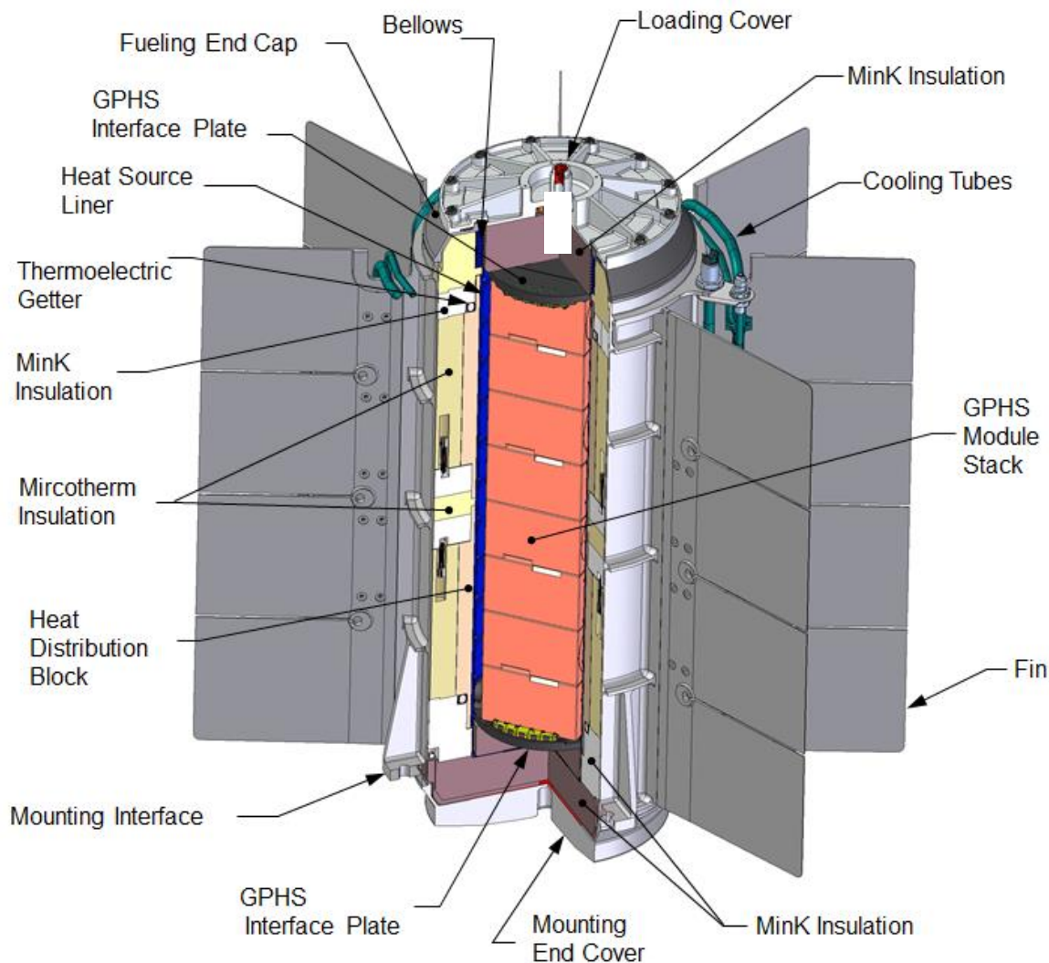
Figure 2-11. MMRTG
