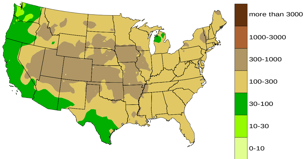
Figure 3.3. Strontium-90 deposition density (Bq/m 2 ) due to all NTS tests.
