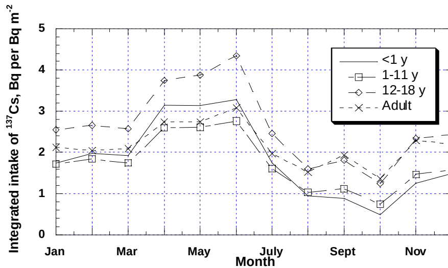
Figure 3.11. Monthly values of integrated intake for four age groups for ^{137}\text{Cs} . Data were derived from Whicker and Kirchner (1987).
