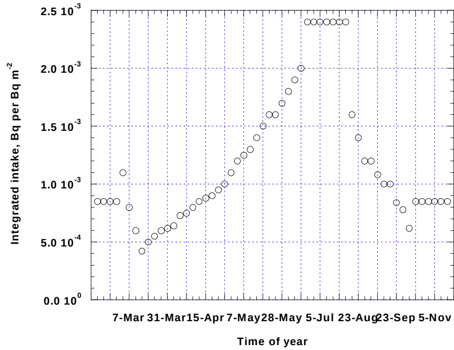
Fig. 16. Values for integrated intake used for 143 Ce.
