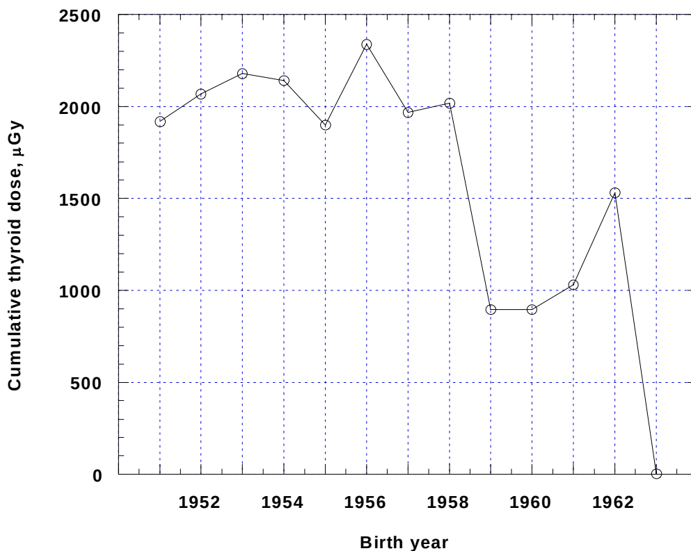
Fig. 26. Cumulative (1953 through 1963) thyroid dose as a function of birth year.
