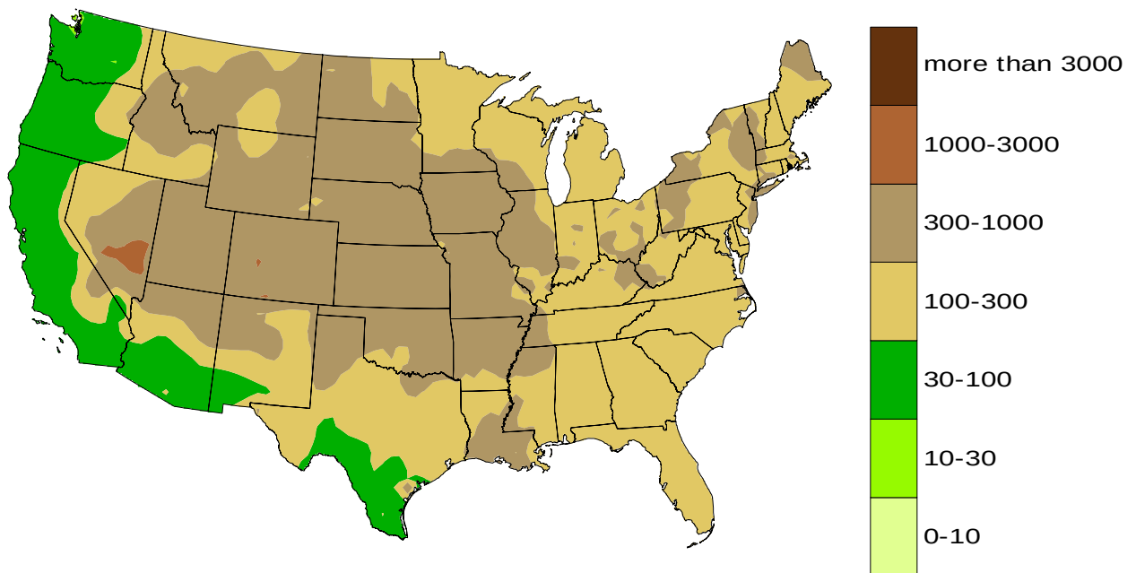
Figure 3.2. Cesium-137 deposition density ( \text{Bq/m}^2 ) due to all NTS tests.
