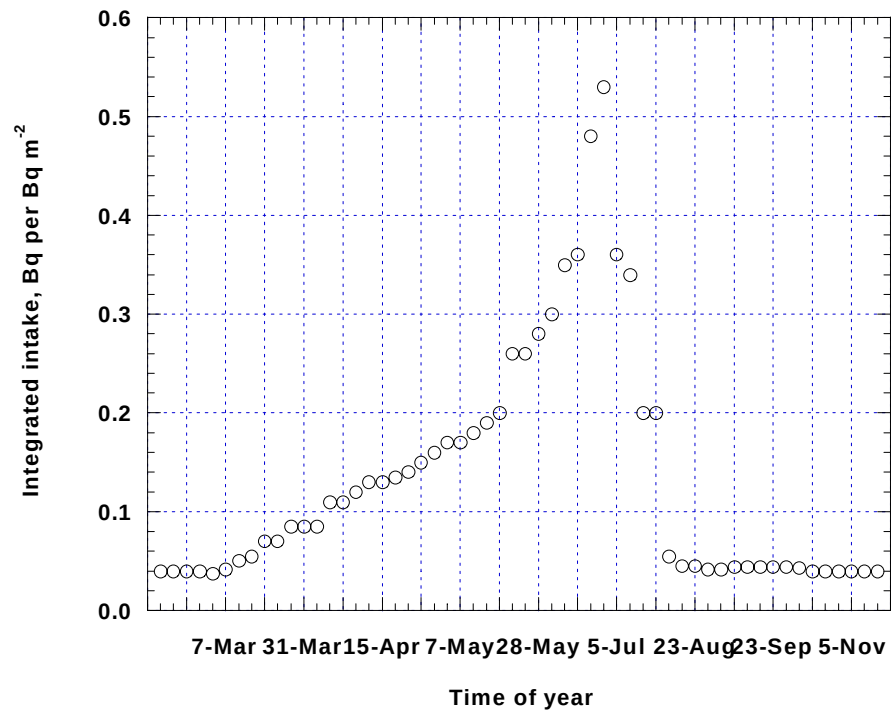
Fig. 17. Values for integrated intake used for 144 Ce.
