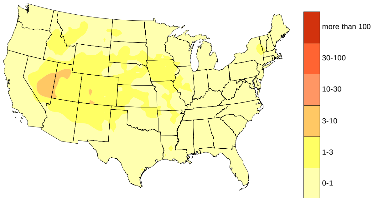
Figure 3.14. Total (external + internal) dose (mGy) to the red bone marrow of adults in 1951 from all NTS tests.
