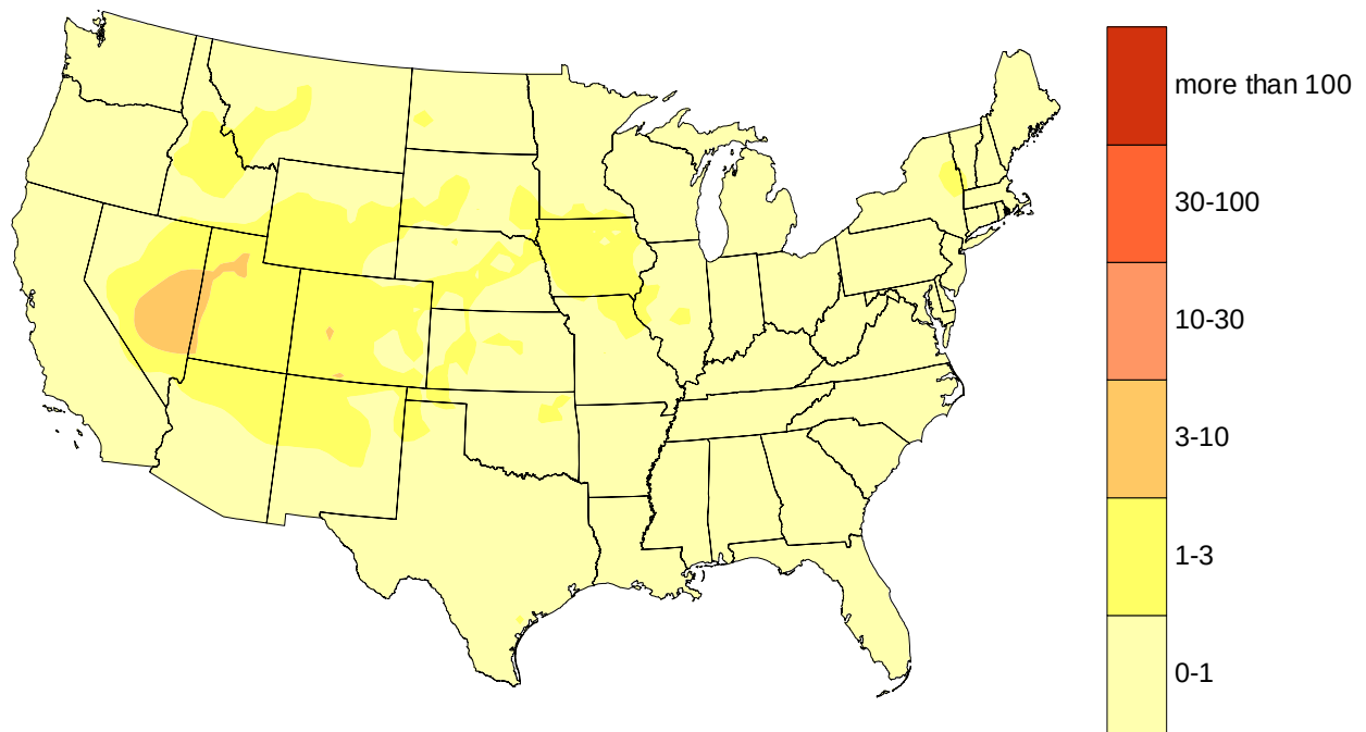
Figure 3.6. External dose (mGy) to the red bone marrow and the thyroid gland for both children and adults resulting from all NTS tests.
