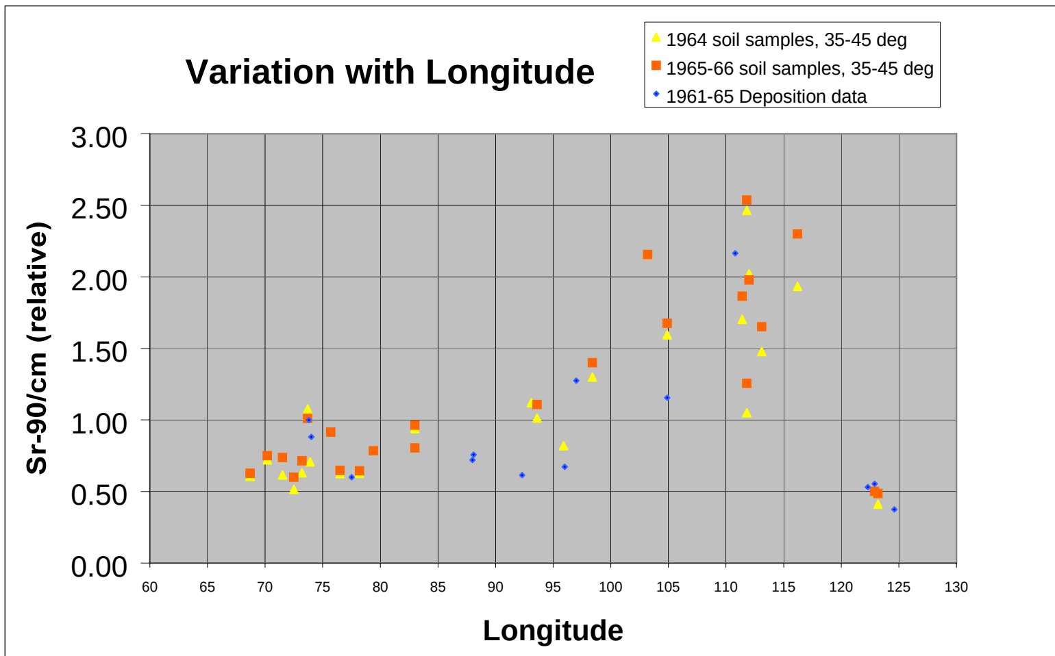
Figure 4: Variation of Sr-90 Deposition Density per cm of rain with longitude. The ordinate values for the deposition data have been normalized to those for the soil data since the soil data represent cumulate deposition at the time of sampling.
