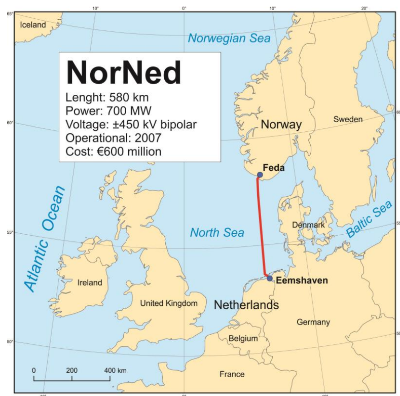
Fig. 39 – NorNed HVDC submarine power cable between Norway and The Netherlands
