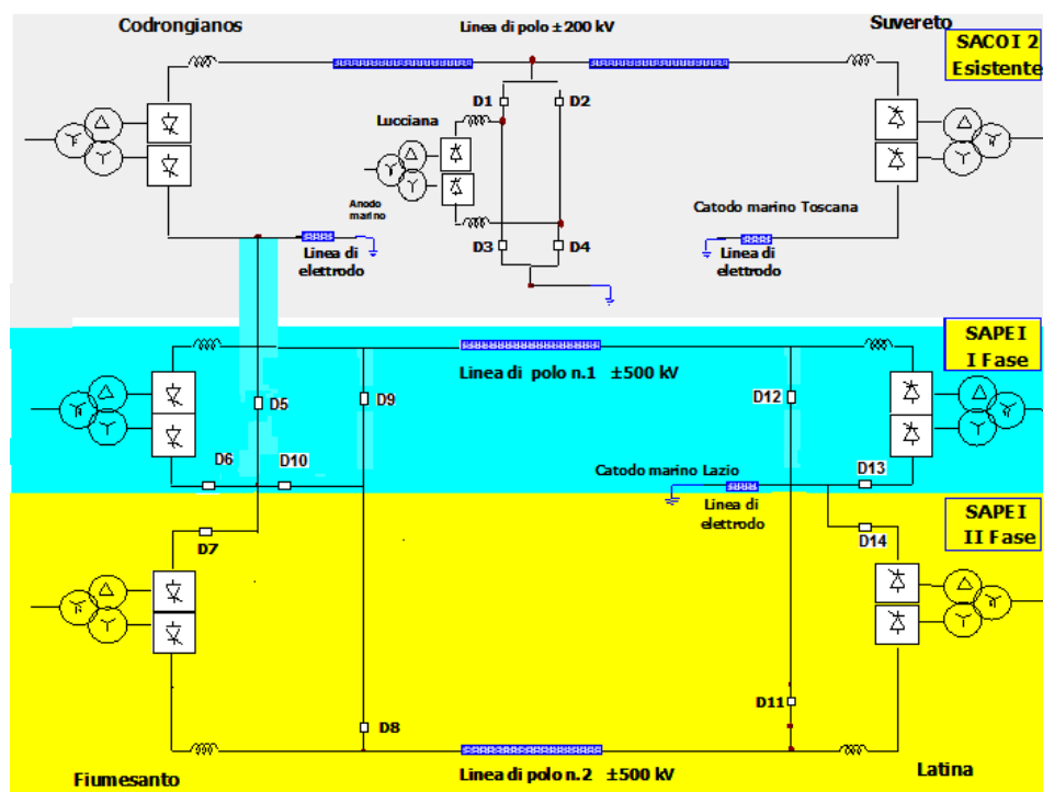
Fig. 44 – The configuration of the SAPEI HVDC interconnector (Rendina et al., 2012)
