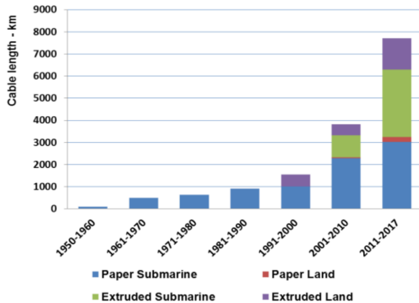
Fig. 28 – Length evolution for mass impregnated paper and extruded power cables in submarine and underground environments (Zaccone, 2014)
