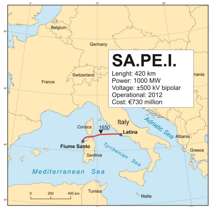
Fig. 40 – SAPEI. HVDC submarine power cable in Italy between Sardinia and the peninsula
