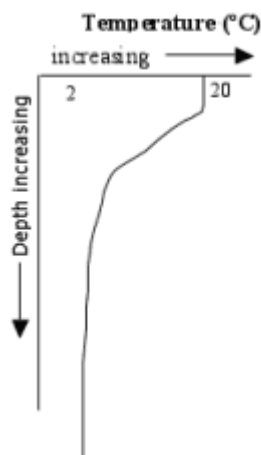
Fig. 21 – Temperature decrease with depth (Source: dosit.org ) Fig. 22 – Salinity increase with depth (Source: dosit.org )
