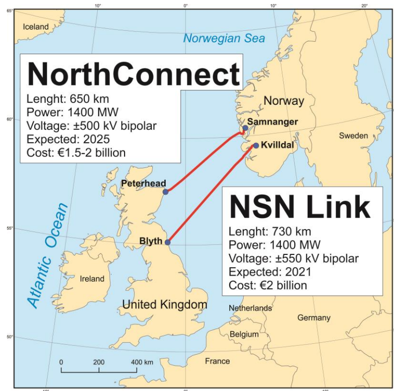
Fig. 46 – Future NSN Link and NorthConnect HVDC submarine power cable routes between Norway and United Kingdom
