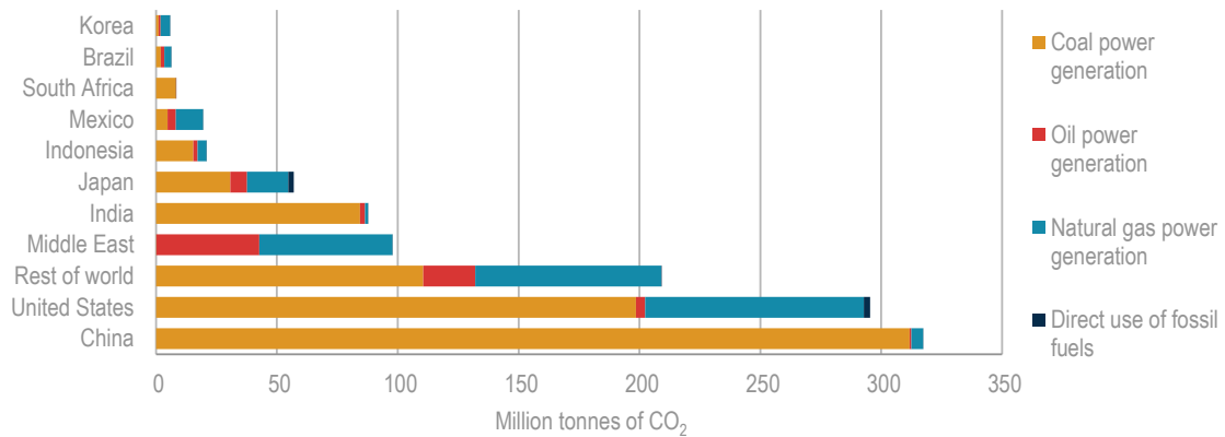
Figure 1.16 • Energy-related CO 2 emissions from space cooling by source and country/region in 2016
