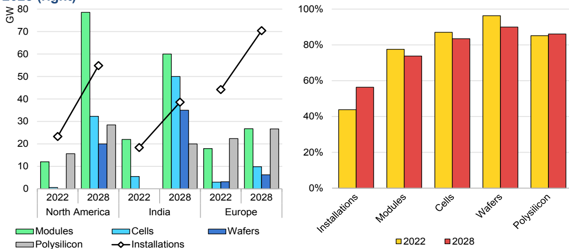
Solar PV manufacturing capacity and annual installations in North America, India and Europe, 2022-2028 (left), and China’s share in PV production and installations, 2022-2028 (right)
