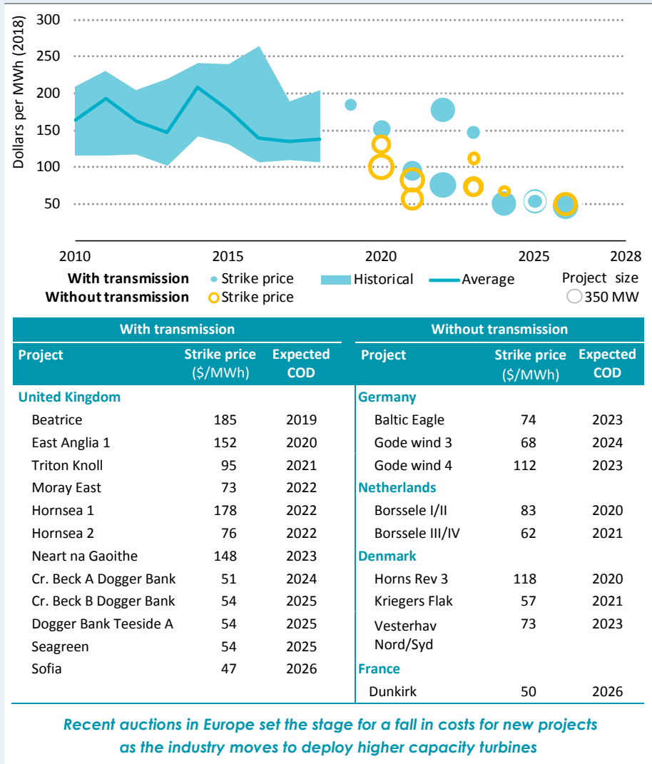
Figure 8 ▶ Historical LCOE of offshore wind and strike prices in recent auctions in Europe
