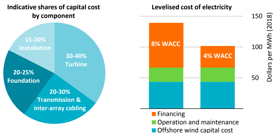
Figure 7 ▶ Offshore wind indicative shares of capital costs by component and levelised cost of electricity for projects completed in 2018
