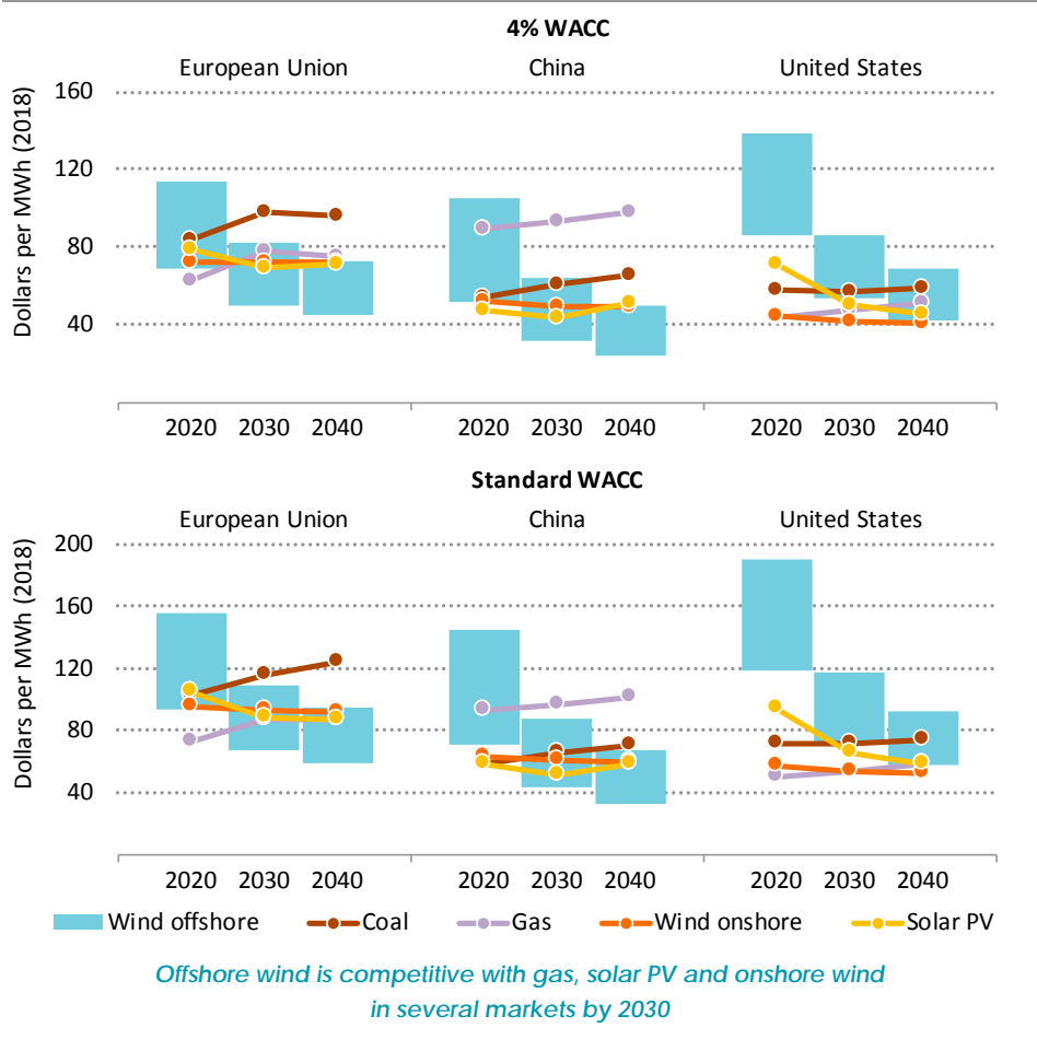
Figure 24 ▶ Evolution of offshore wind competitiveness: value-adjusted LCOEs by technology and region in the Stated Policies Scenario
