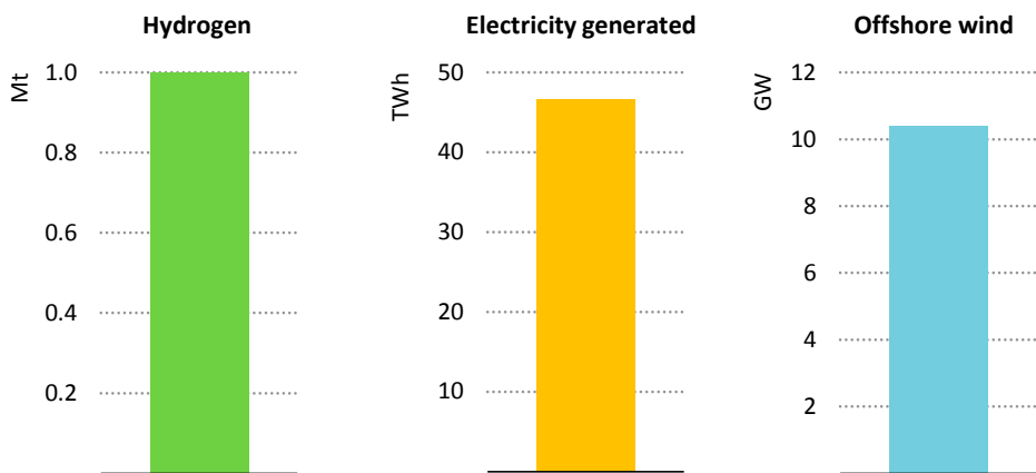
Figure 29 ▶ Offshore wind capacity needed to produce 1 Mt of hydrogen
