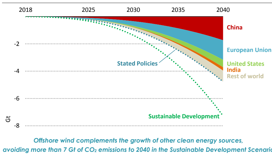
Figure 32 ▶ Avoided CO 2 emissions due to the deployment of offshore wind in the Stated Policies and Sustainable Development scenarios
