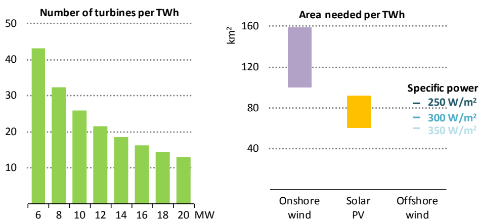
Figure B.3 ▶ Number of turbines and space requirements
