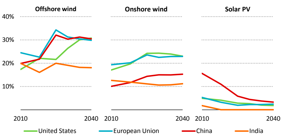
Figure 23 ▶ Average capacity credit by technology and region in the Stated Policies Scenario
