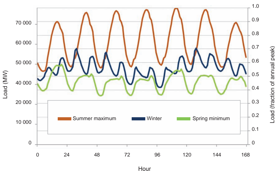
Figure 2.1: Hourly electricity demand curve in Texas (ERCOT) for 3 weeks in 2005
