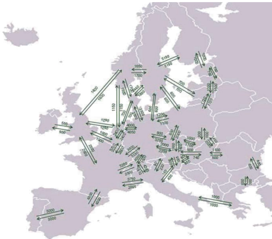
Figure 5.2: European objectives for interconnection capacity in 2020 (MW, PRIMES Reference Scenario)
