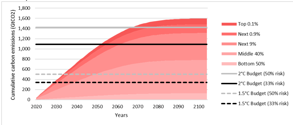
Figure 13(a,b, c, d): Global cumulative emissions associated with the consumption of individuals in different global income groups from 2020 for the SSP1 and SSP4, and RCP6.0 and RCP1.9 scenarios. The horizontal lines reflect the remaining budget for 1.5°C (dashed) and 2°C (solid) warming levels, each with a 50% (grey) and 33% (black) risk of failure.
