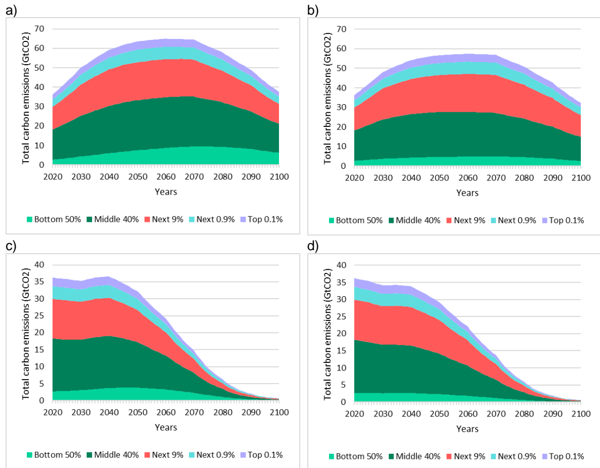
Figure 12(a, b, c, d): Total carbon emissions associated with the consumption of individuals in different global income groups from 2020 for the SSP1 (left) and SSP4 (right), and RCP6.0 (upper) and RCP1.9 (lower) scenarios.
