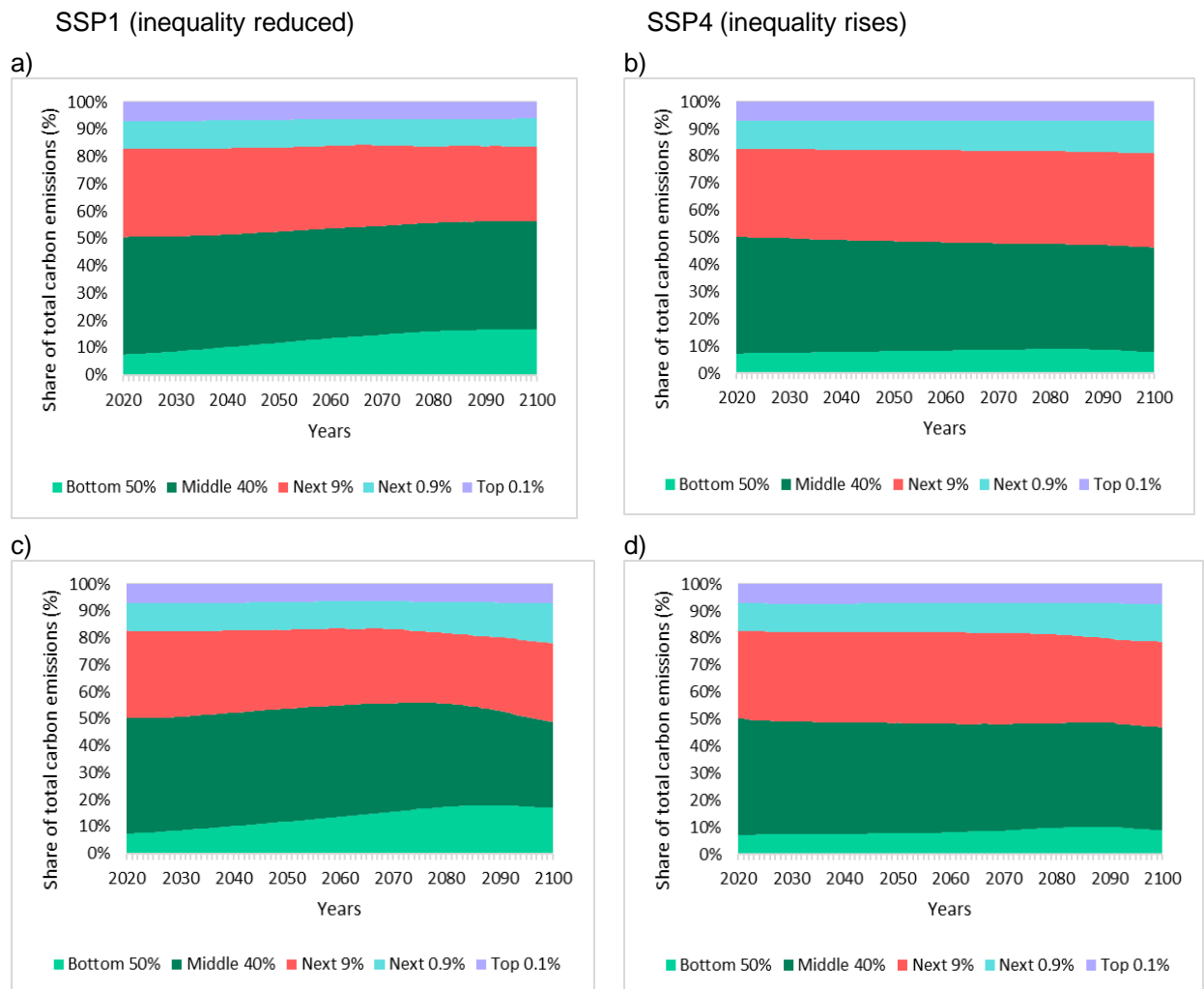
Figure 11(a, b, c, d): Share of total carbon emissions associated with consumption of individuals in different global income groups for the SSP1 (left) and SSP4 (right), and RCP6.0 (upper) and RCP1.9 (lower) scenarios.
