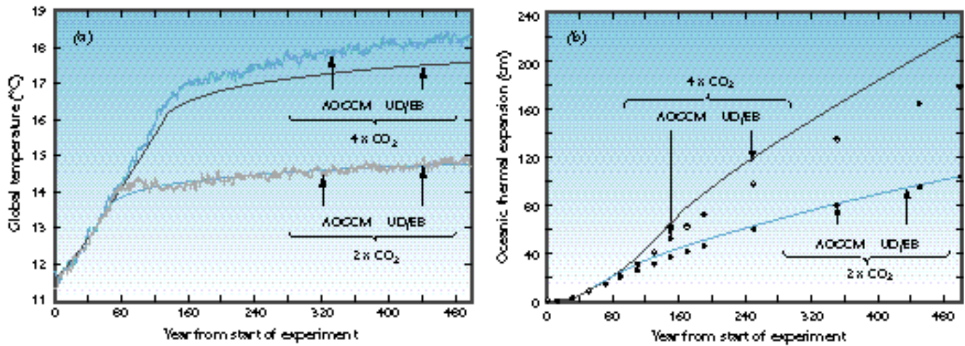
Figure 17. Comparison between the AOGCM results of Manabe and Stouffer (1994) and the one-dimensional upwelling-diffusion model for cases in which the atmospheric CO 2 concentration increases by 1 per cent per year (compounded) until the concentration has either doubled or quadrupled and is then stabilized (a) global mean surface air temperature; (b) sea level rise due to ocean thermal expansion (reproduced from SAR WGI, Figure 6.17).
