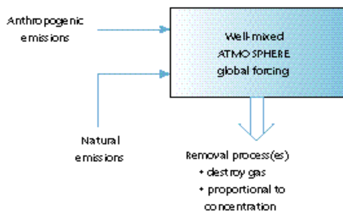
Figure 6. Schematic illustration of the treatment of well-mixed gases ( CH_4 , N_2O , halocarbons) in simple climate models. The removal rate is linearly proportional to concentration in the case of N_2O and halocarbons, but varies non-linearly with atmospheric concentration in the case of CH_4 .
