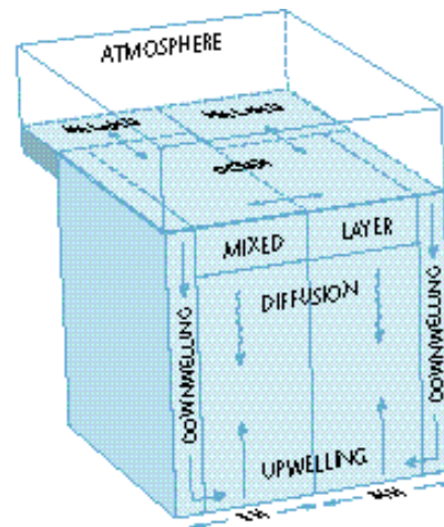
Figure 9. Illustration of a variant of the one-dimensional upwelling-diffusion model having separate land and sea boxes within each hemisphere, and separate polar sinking and upwelling in each hemisphere. This variant was used in the SAR WGI (Section 6.3 and 7.5.2).
