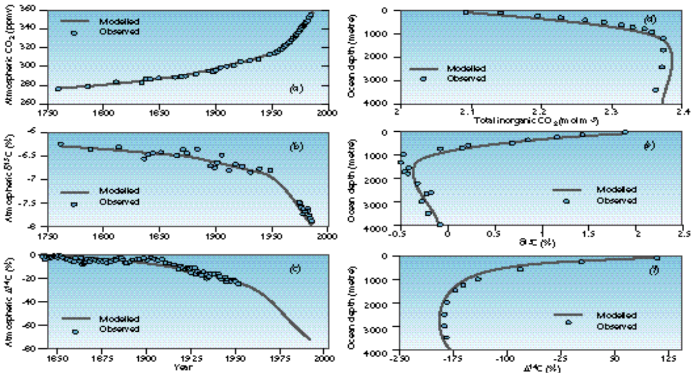
Figure 5. Comparison of observed and model-simulated historical variation of (a) atmospheric CO 2 concentration; (b) atmospheric 13 C (a measure of the ratio of 13 C to total C ratio); (c) atmospheric 14 C (a measure of the ratio of 14 C to total C ratio); and observed and model-simulated vertical profiles of (d) total dissolved carbon (e) 13 C, and (f) 14 C as simulated by the carbon cycle model of Jain, et al. (1995).
