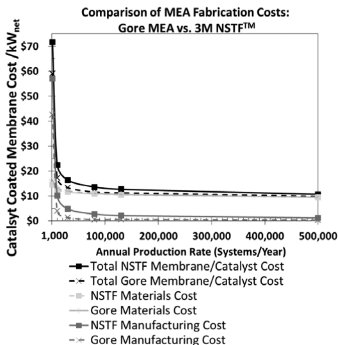
FIGURE 1. Cost Comparison of Gore and 3M MEAs
