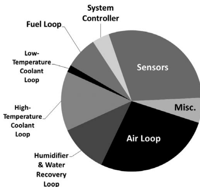
FIGURE 3. Cost Break-Down for PEM Fuel Cell Bus BOP
