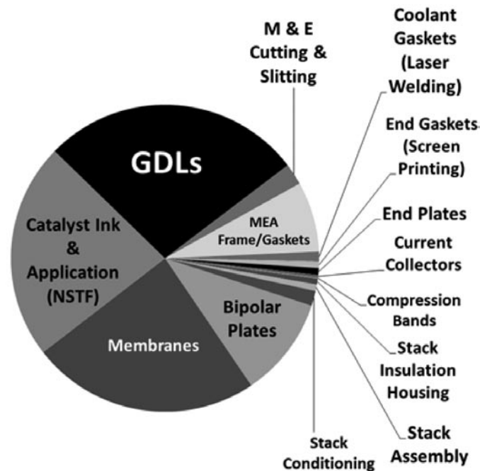
FIGURE 2. Cost Break-Down for PEM Fuel Cell Stacks for a Bus
