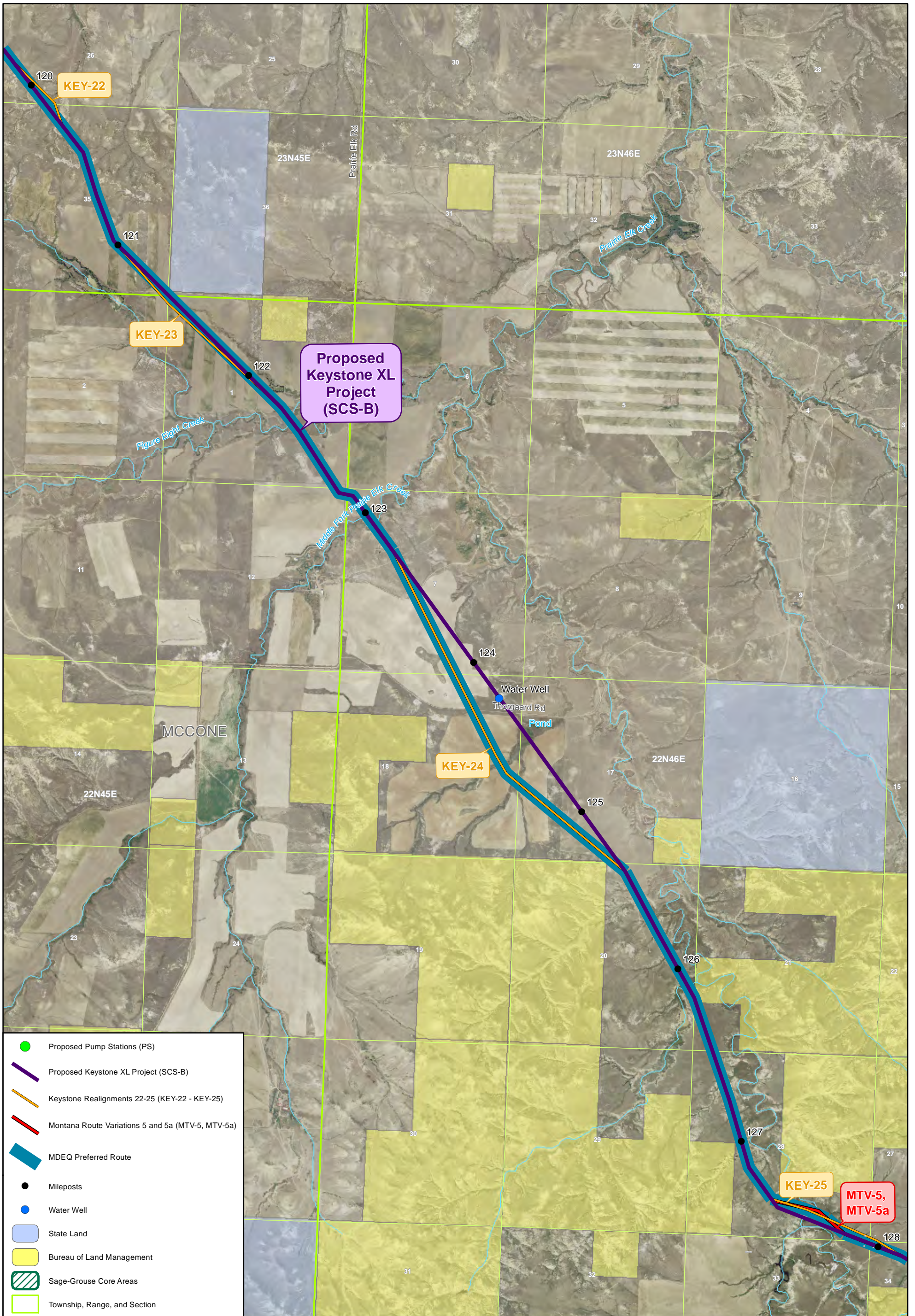
Figure I-2.4.3-12 Keystone Realignments 22-25 (KEY-22 - KEY-25)
