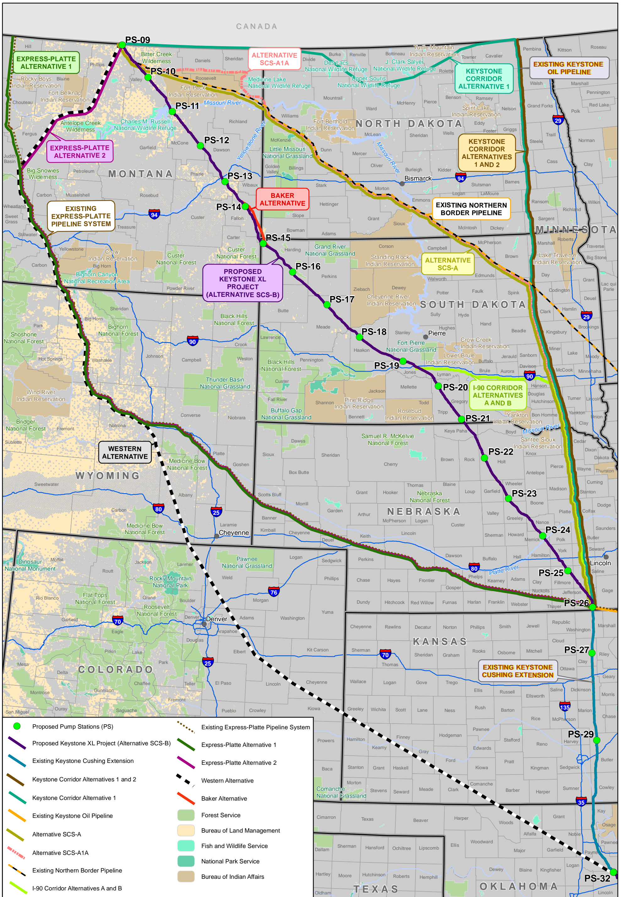
Figure 4.3.3-1 Steele City Segment Alternatives
