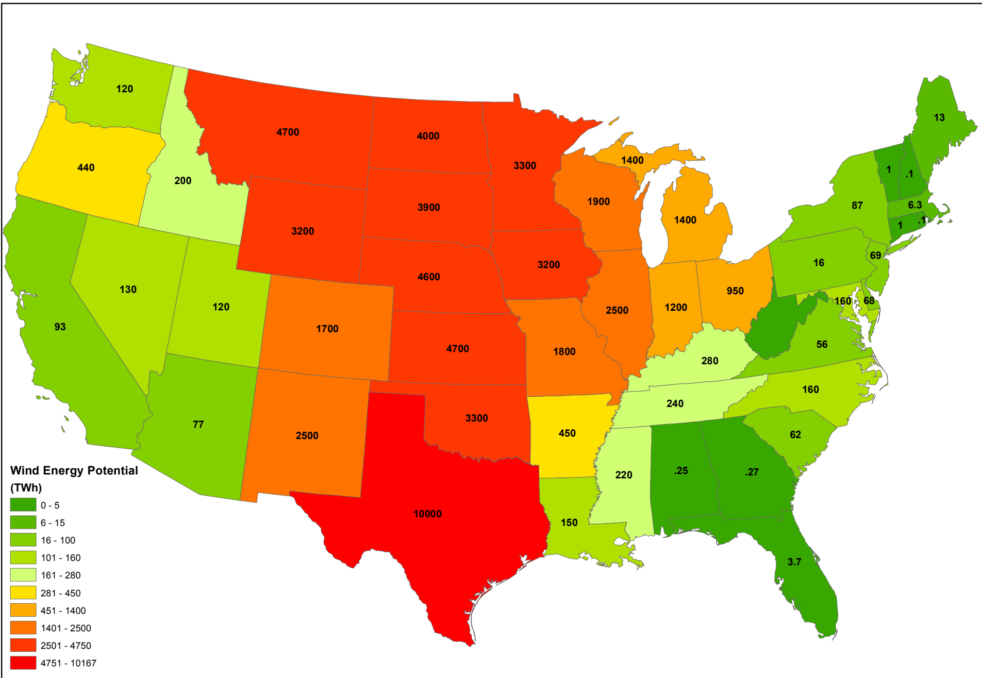
Figure 3.14.2-6 Annual Onshore Wind Energy Potential
