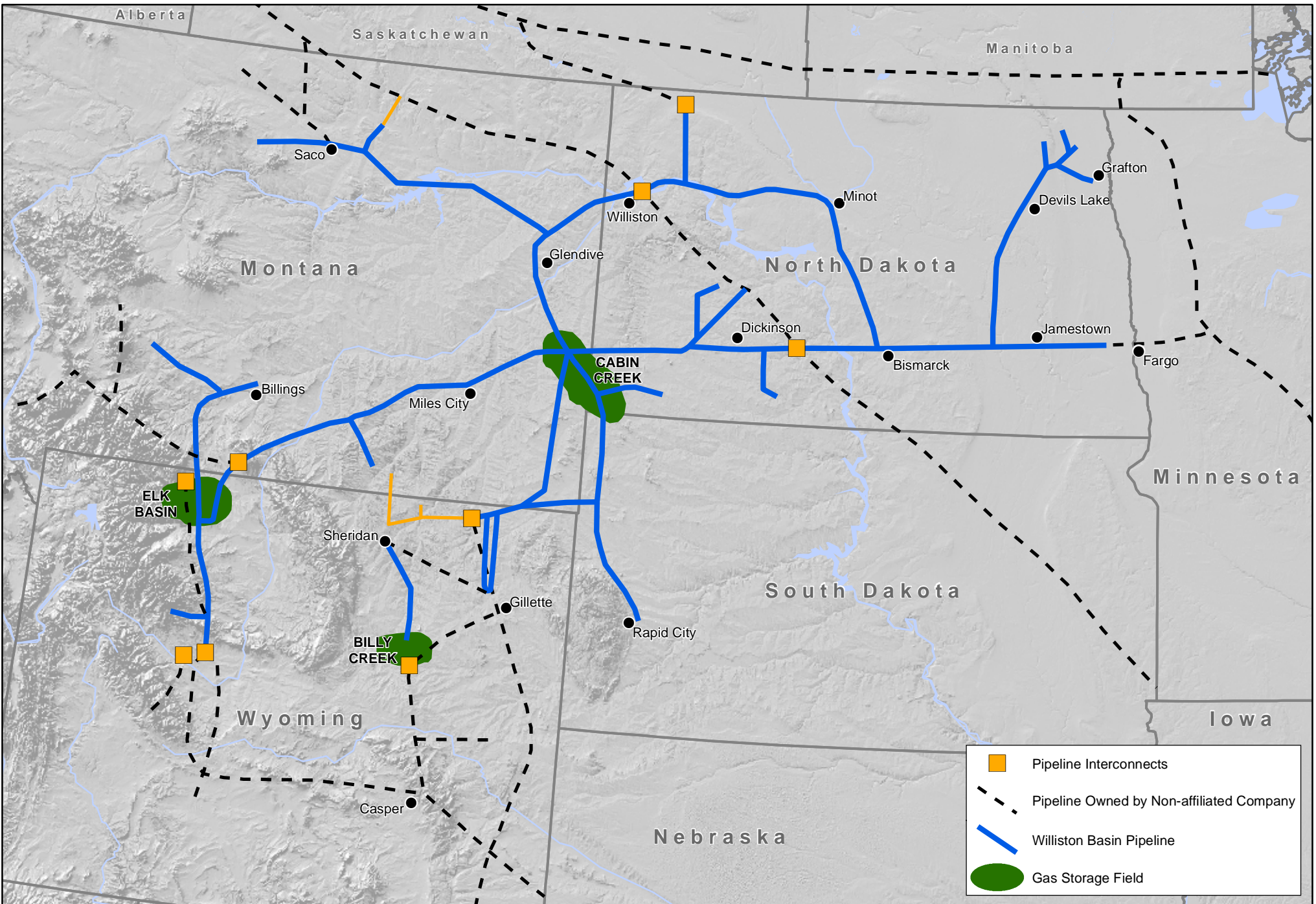
Figure 3.14.2-3 Williston Basin Pipeline
