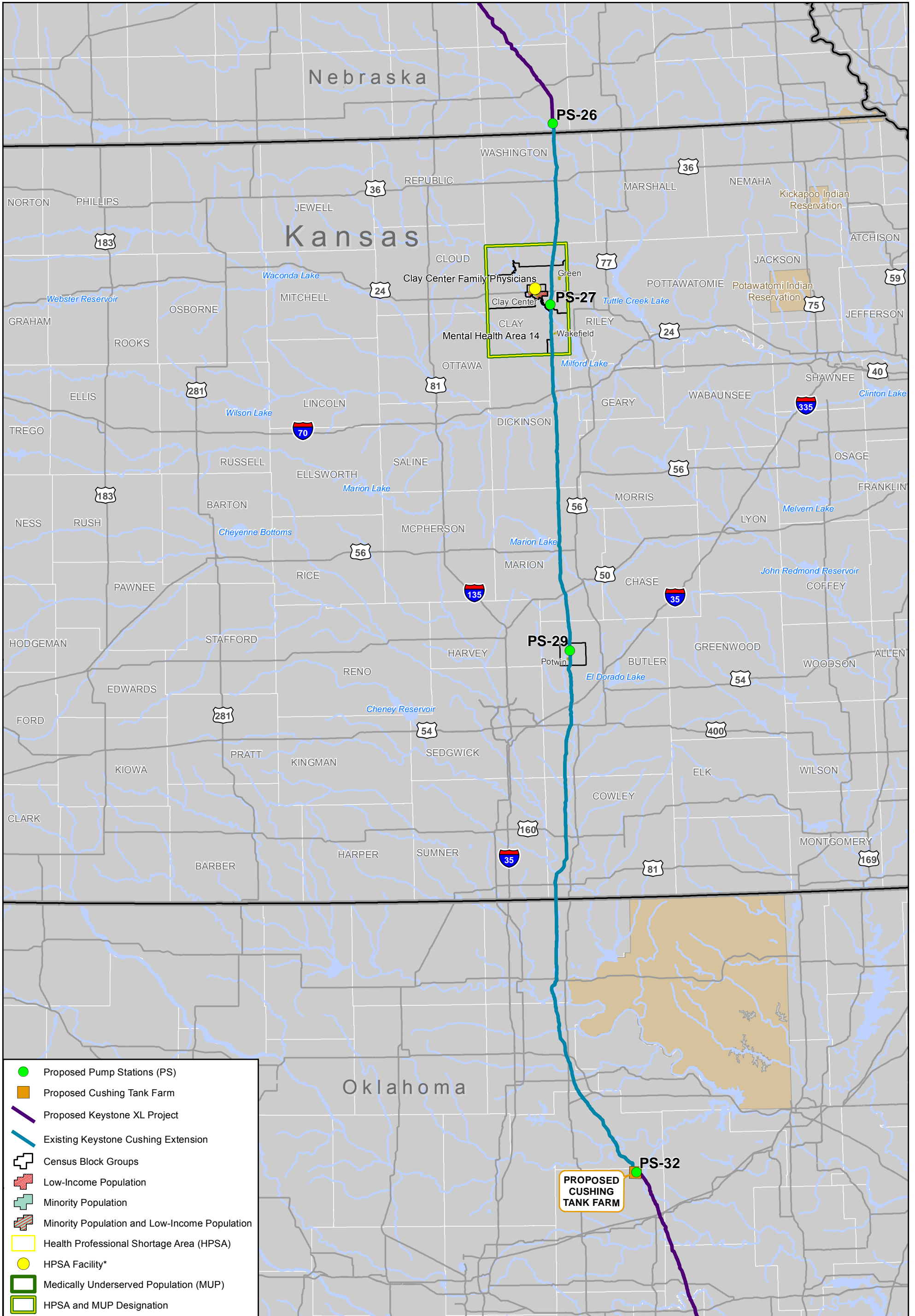
Figure 3.10.1-10 Environmental Justice Analysis - HPSA and MUP Designations (Kansas)
