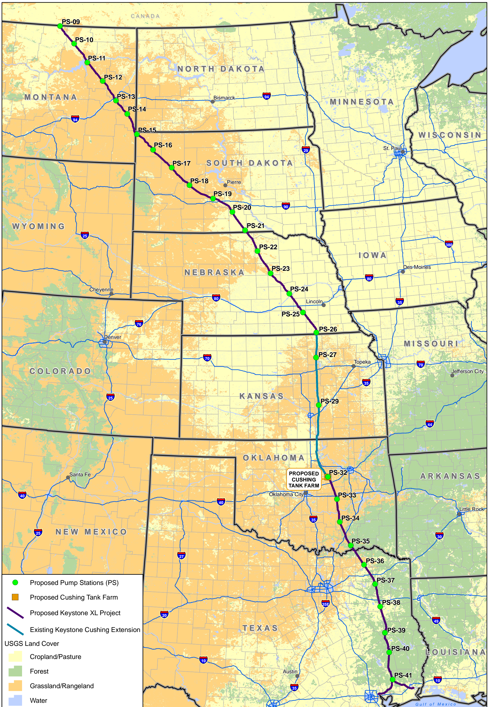
Figure 3.5.2-1 USGS Land Cover
