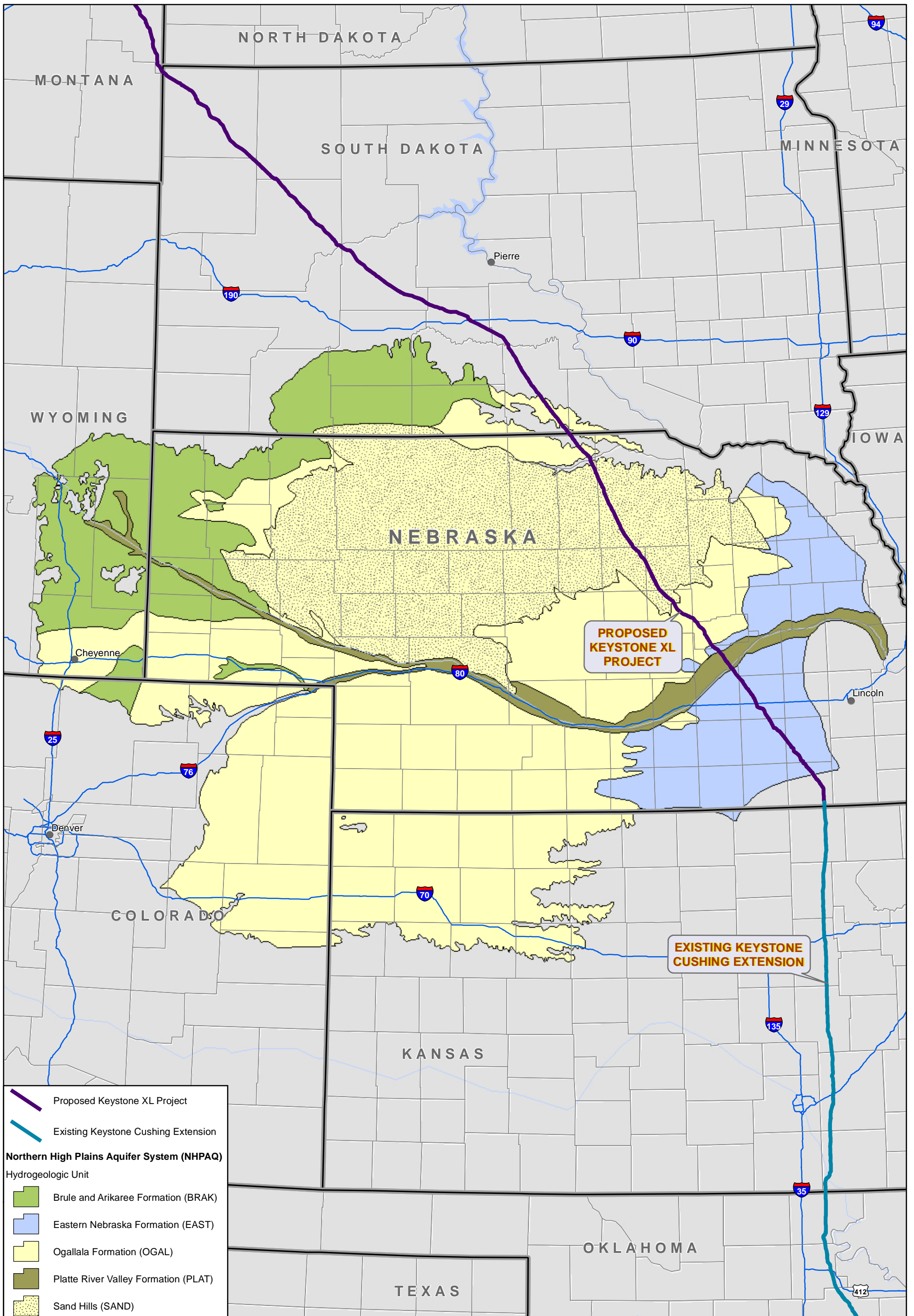
Figure 3.3.1-6 Northern High Plains Aquifer System Hydrogeologic Units
