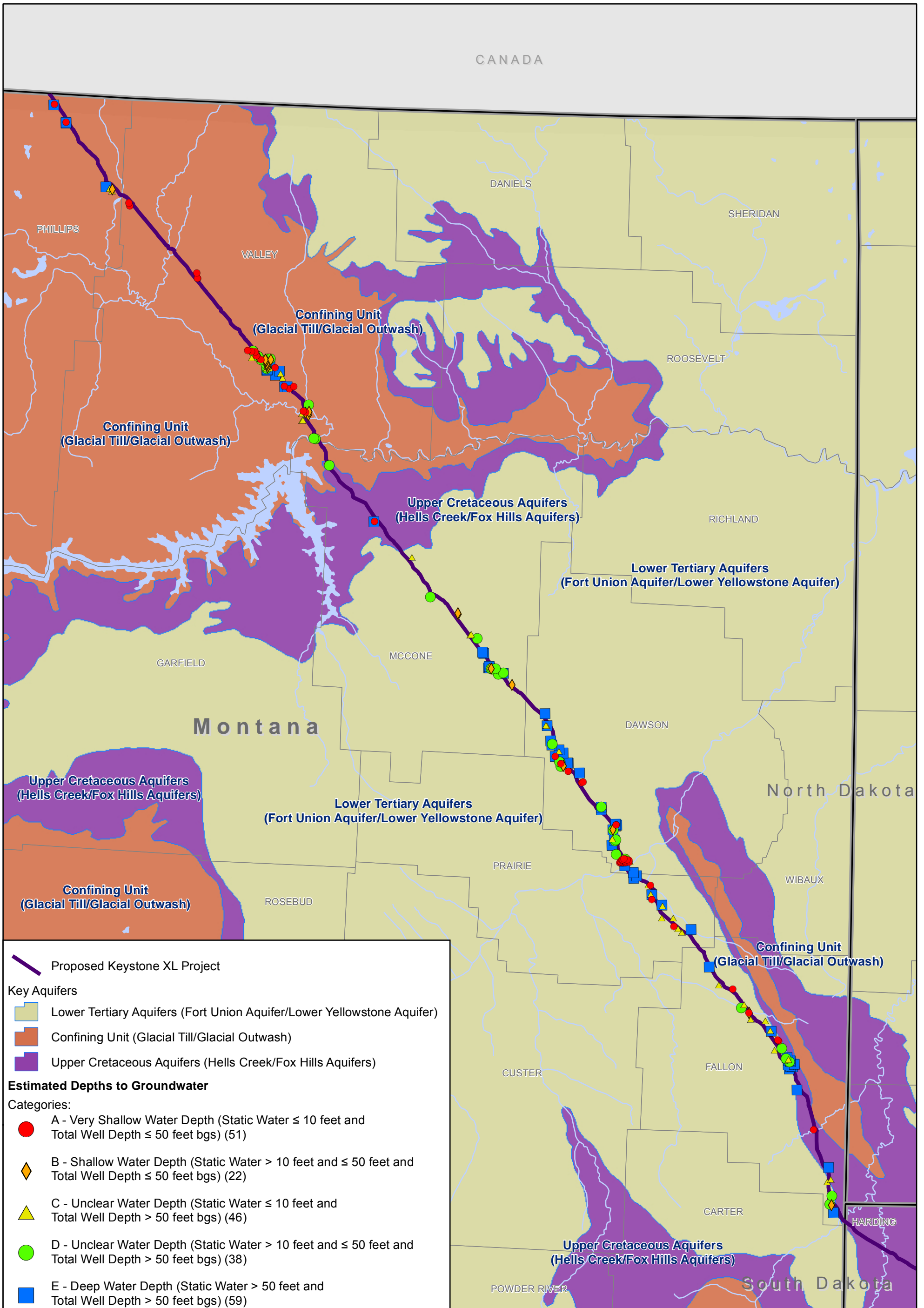
Figure 3.3.1-1 Key Aquifers and Potable Water Wells within 2-mile Corridor (Montana)
