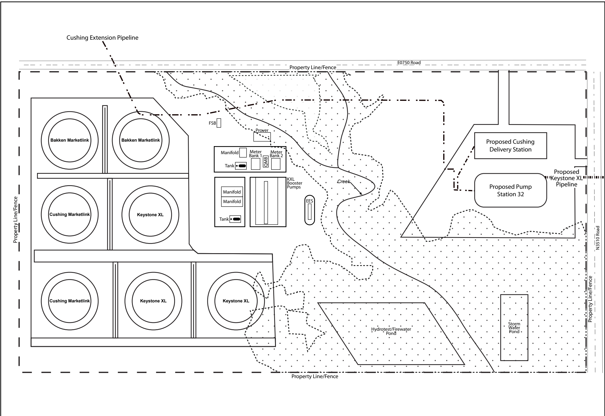
Figure 2.5.3-4 Cushing Tank Farm Proposed Plot Plan with Marketlink Project Facilities
