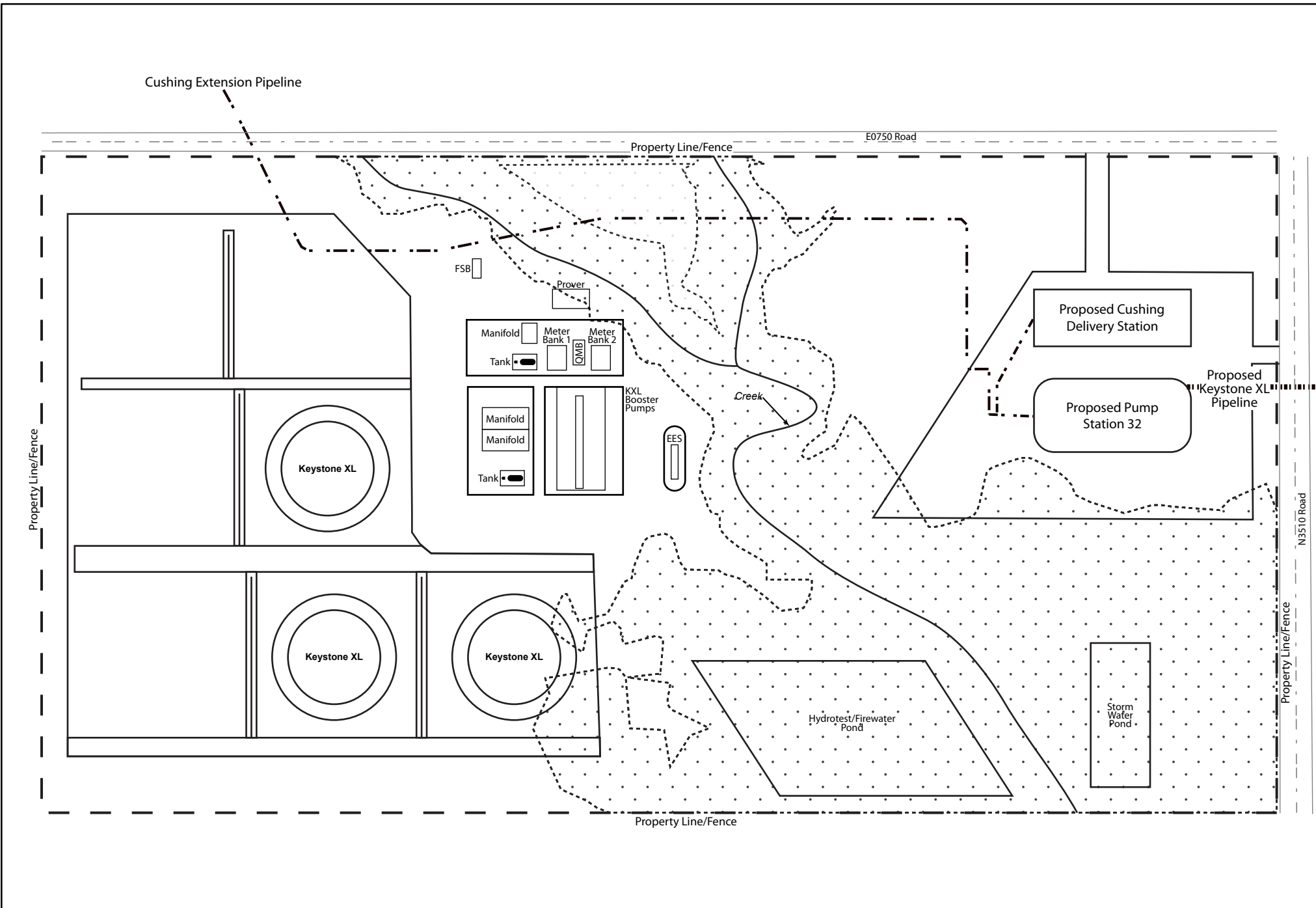
Figure 2.2.6-1 Cushing Tank Farm Proposed Plot Plan
