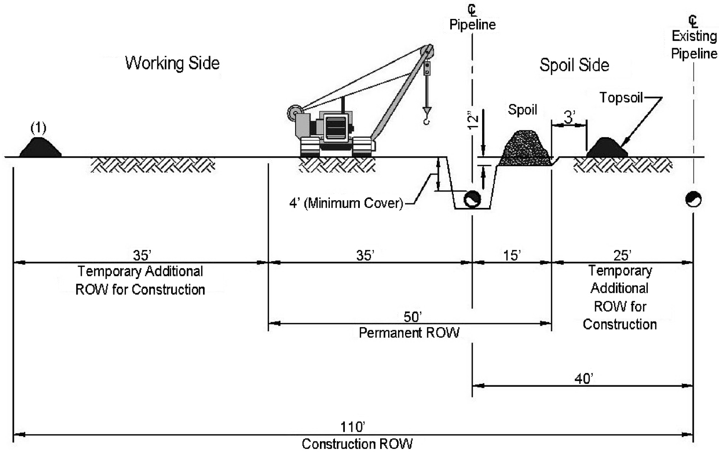
(1) Alternate Topsoil Placement Locations
